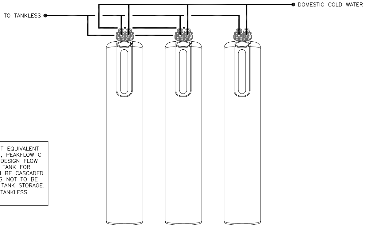
FRONT VIEW
