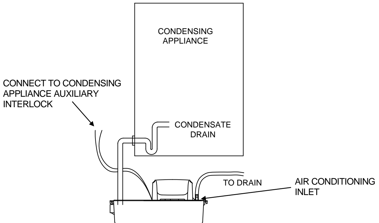
Figure 4: Installation Diagram of the Residential Neutralizer Tank with Pump
